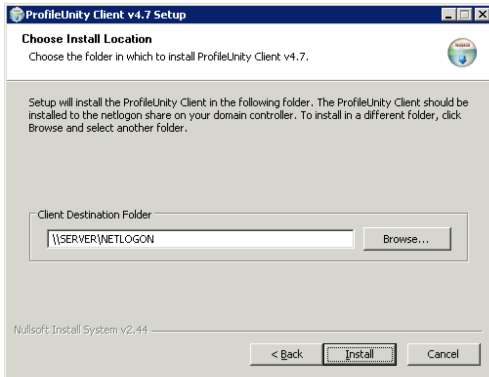
Figure 1.2.2: Client Destination Folder
