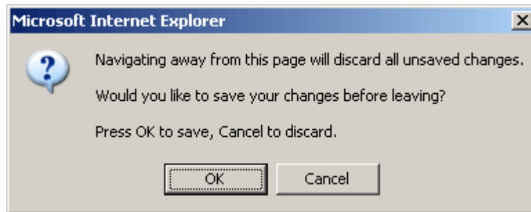
Figure 3.1.2: Save Warning
